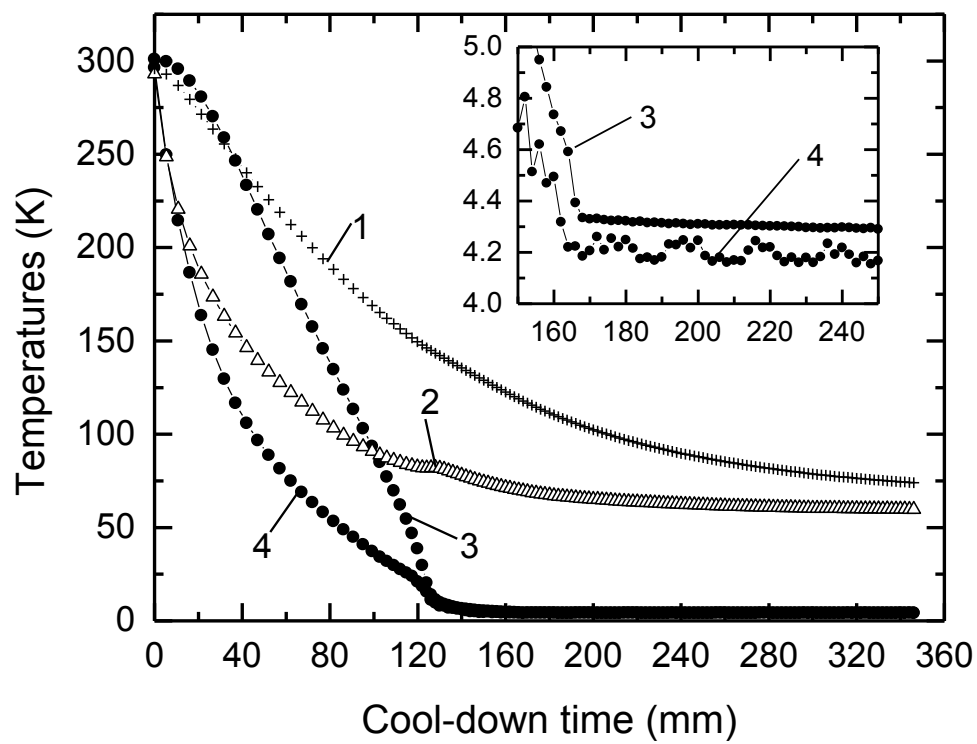
Cool-down curve of the system. 1. radiation shield; 2, 1 st stage heat exchanger/condenser; 3. sample cooling station; 4. 2 nd stage heat exchanger/condenser.
